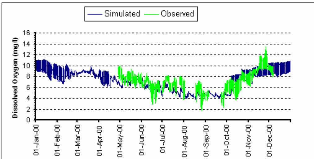
Figure 3.6: DO in the Old River at DMC.
