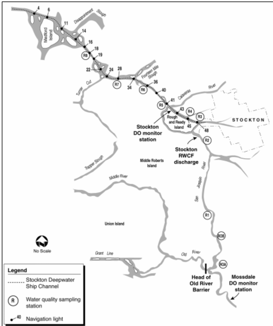
Figure 3.1: Water Quality Stations near Stockton. (Adapted from Jones and Stokes, 2001)
